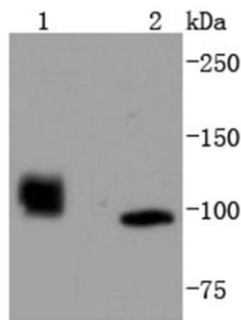
Fig. 1. Western blot analysis of HDAC7 on different lysates using anti-HDAC7 antibody at 1/1,000 dilution. Positive control: Lane 1: A549; Lane 2: Human brain
